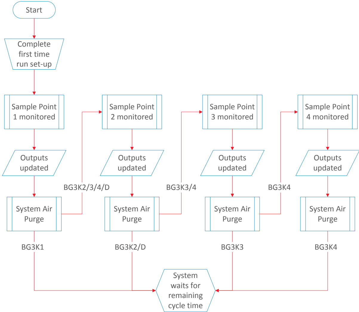
Flow Chart 1 - BG3K1, 2, 3, 4, and D
