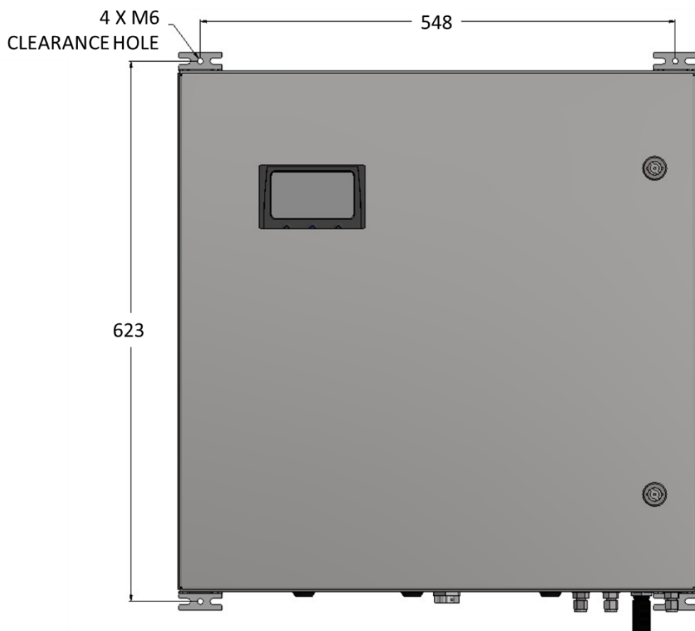
Figure 4 - BIOGAS 3000 enclosure dimensions
