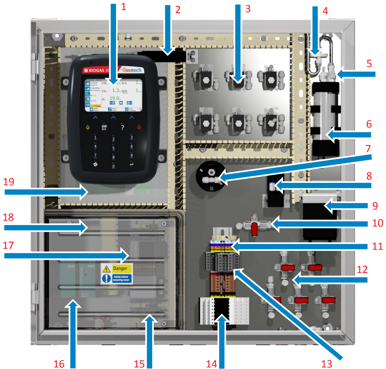
Figure 2 - BIOGAS 3000 internal components
